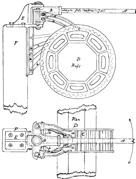
Fig. 12. Lindahl &amp; Runers ankarspel
